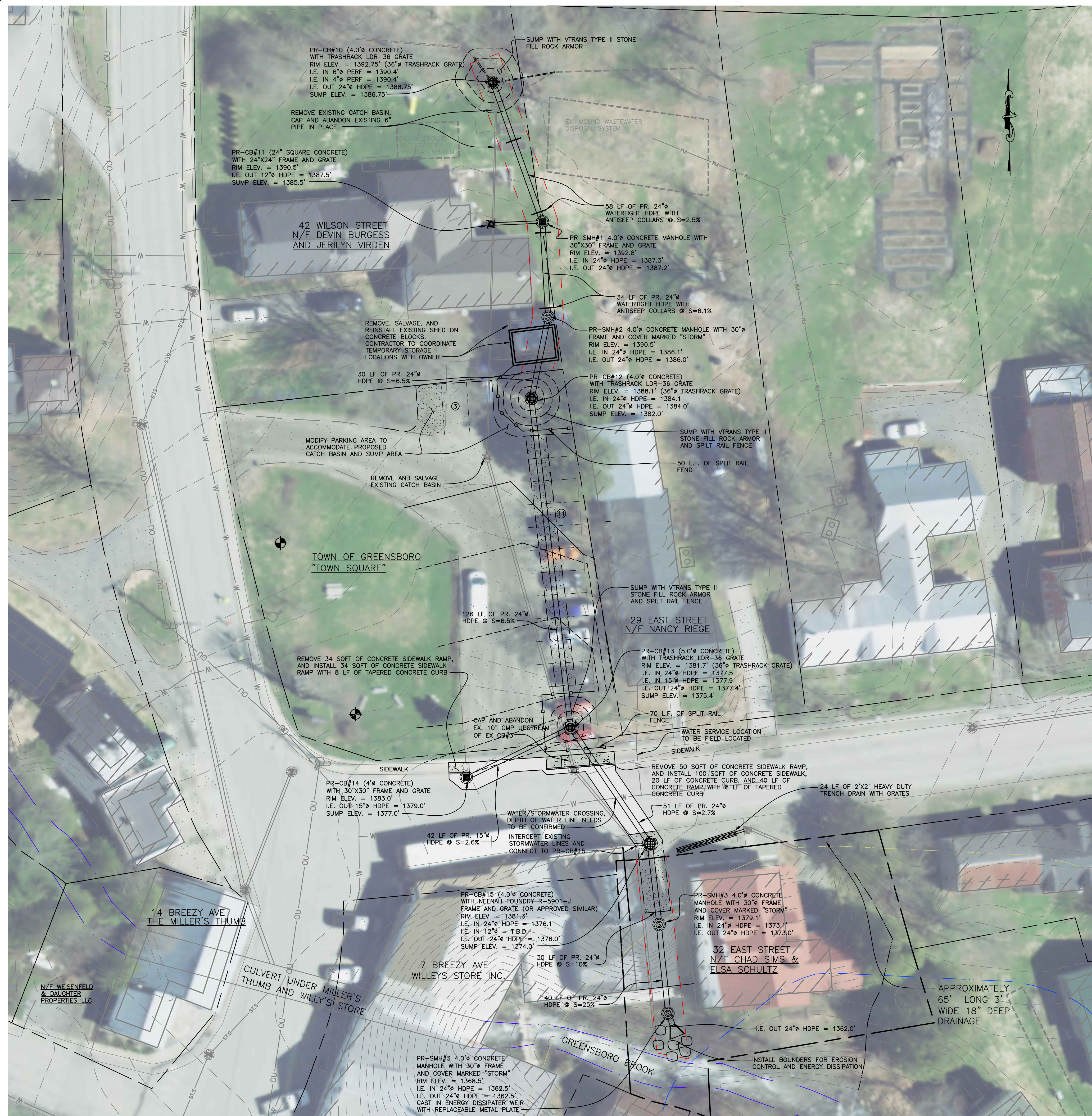
WILSON STREET STORMWATER PROPOSED ALTERNATIVE 1 SCALE 1"=20'
